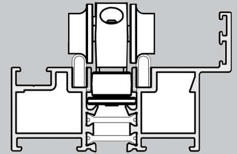
Retained roller guides
